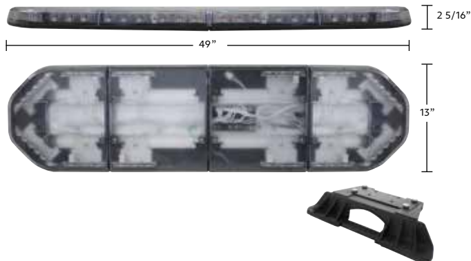
Standard Bolt / Strap Mount
